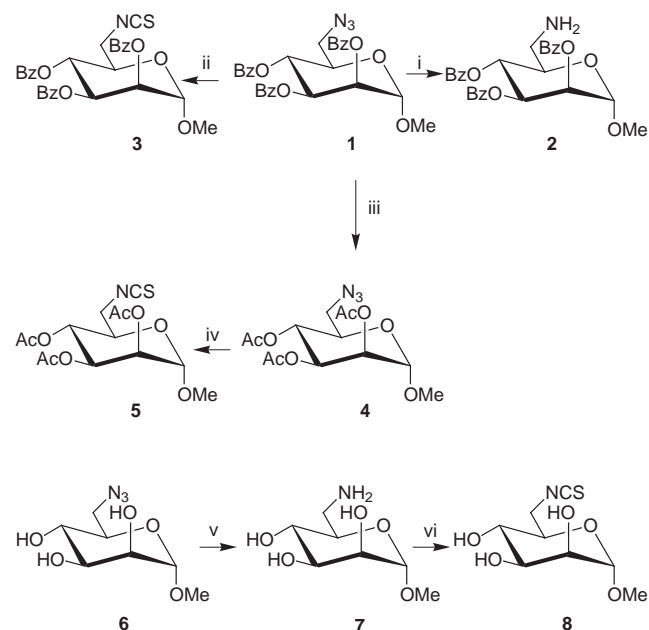
Scheme 1 Reagents, conditions and yields: i, \text{H}_2 , Pd/C (10%), 1:1 EtOAc–EtOH, rt, 89%; ii, \text{CS}_2 , (\text{EtO})_3\text{P} , toluene, 80 °C, 4 h, 92%; iii (a) NaOMe, MeOH; (b) \text{Ac}_2\text{O} , pyridine, rt, 90%; iv, \text{CS}_2 , (\text{EtO})_3\text{P} , toluene, 80 °C, 6 h, 87%; v, \text{H}_2 , Pd/C (10%), 1:1 EtOAc–EtOH, 84%; vi, \text{Cl}_2\text{C}(\text{S}) , 4:1 EtOH–water, diisopropylethylamine, rt, 96%
