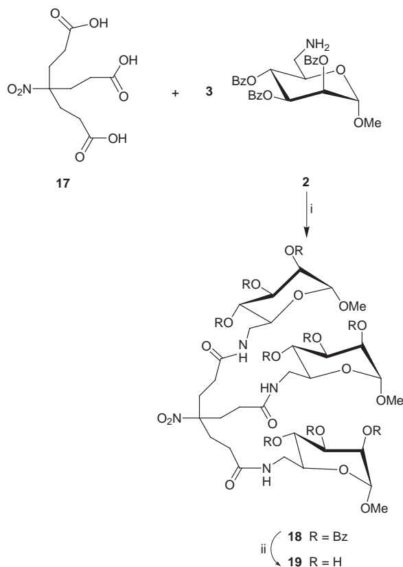
Scheme 4 Reagents, conditions and yields: i, DCC, HOBT, DMF, 0^\circ\text{C} to rt, 73%; ii, NaOMe, MeOH, 98%
