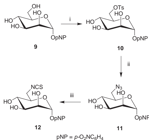
Scheme 2 Reagents, conditions and yields: i, TsCl, pyridine, 0 °C to rt, 57%; ii, \text{NaN}_3 , DMF, 70 °C, 8 h, 91%; iii, \text{CS}_2 , (\text{EtO})_3\text{P} , DME, 80 °C, 6 h, 76%
