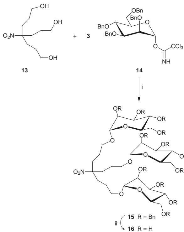
Scheme 3 Reagents, conditions and yields: i, 0.02 M TMSOTf in \text{CH}_2\text{Cl}_2 , THF, 4 Å, \text{N}_2 , -65^\circ\text{C} to rt, 74%; ii, \text{H}_2 , Pd/C, 3:1 EtOH-THF, 77%
