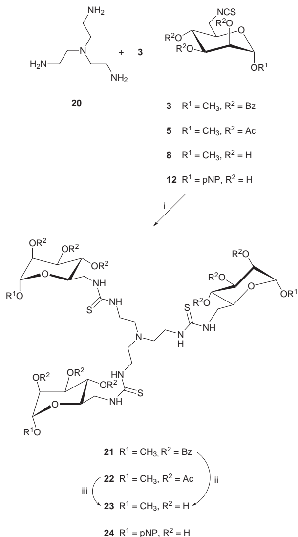
Scheme 5 Reagents, conditions and yields: i, \text{CH}_2\text{Cl}_2 , 50^\circ\text{C} , 30 min (for 3 , 5 or 12 ), 92% ( \text{R}^1 = \text{CH}_3 , \text{R}^2 = \text{Bz} ), 91% ( \text{R}^1 = \text{CH}_3 , \text{R}^2 = \text{Ac} ), 89% ( \text{R}^1 = \text{pNP} , \text{R}^2 = \text{H} ); 4:1 EtOH-water, 50^\circ\text{C} , 12 h, (for 8 ), 23%; ii, 1 M NaOMe, 5:1 MeOH-DMF, 50^\circ\text{C} , 3 days, 27%; iii, 1 M NaOMe, MeOH, rt, 82%
